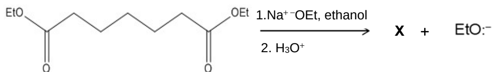
diethyl heptanedioate
